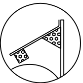
DETAIL A - ALTERNATIVE *C/W MONOFILAMENT OPTION ONLY* SUPER SNUG 'ST' STYLE *ADD 6" TO INWARD PROU'N FOR SUPER SNUG*
